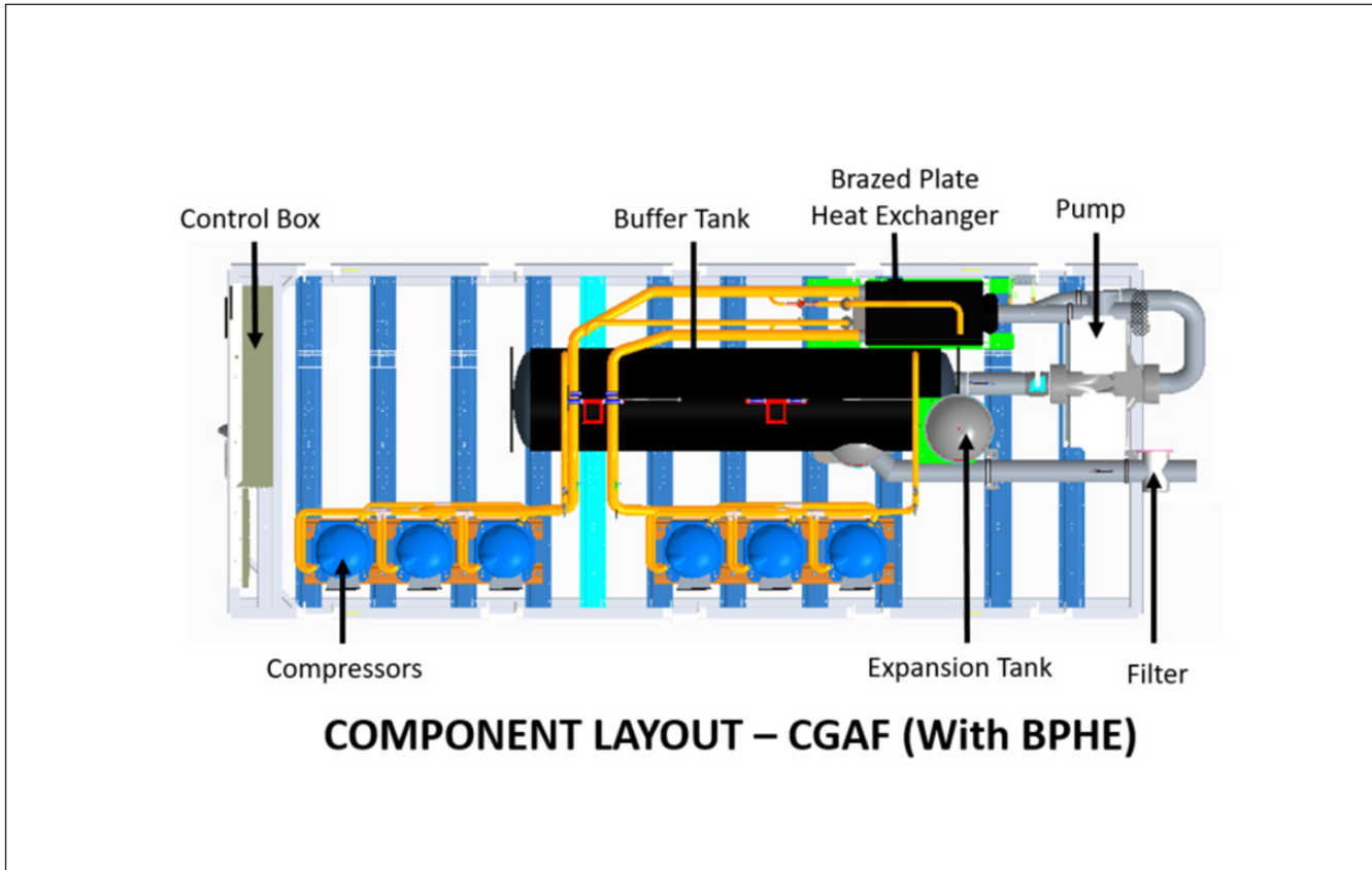
Top view
