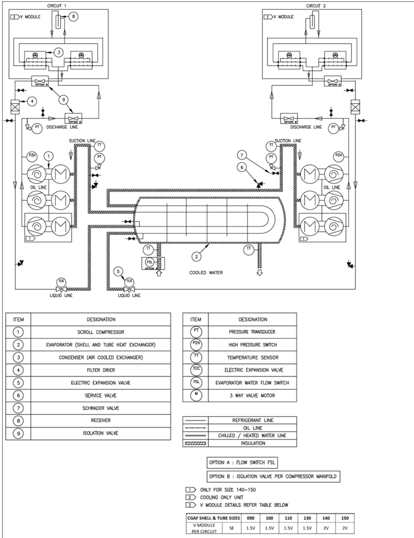
Figure 10 – Example of Typical Refrigerant System Schematic & Oil Lube Circuit Schematic for CGAF S&T
