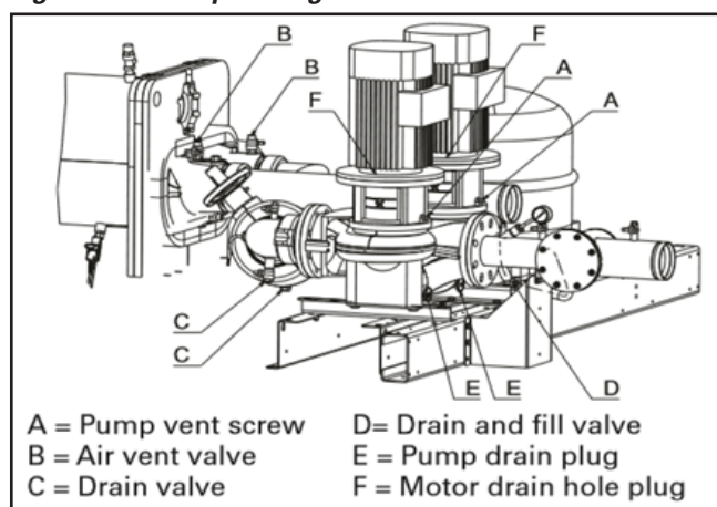
Figure 27 – Pump Package
