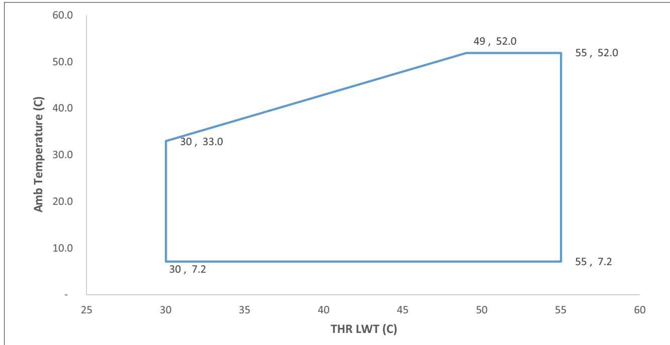
Figure 17 – Total Heat Recovery Operating Map
