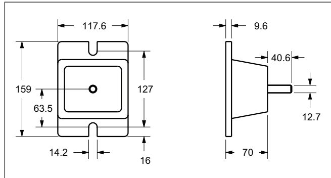
Figure 2 – Elastomeric Isolator
