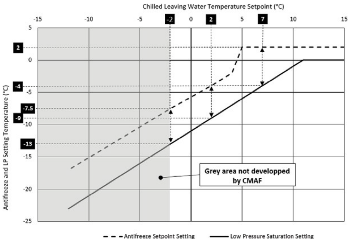
Figure 15 - LP setting Vs. Leaving Water Temperature set point
