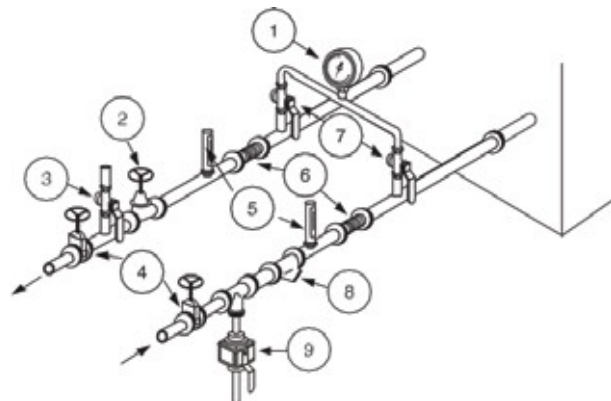
Figure 5 - Unit typical water circuit
