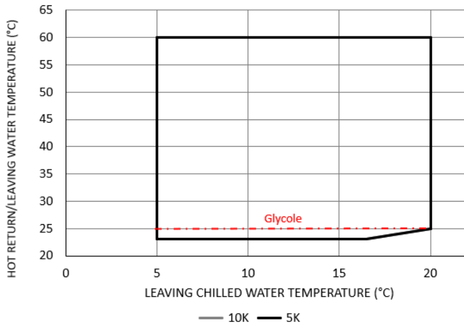
Figure 20 - Heat Recovery operating map
