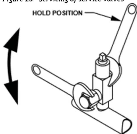
Figure 23 - Servicing of service valves
