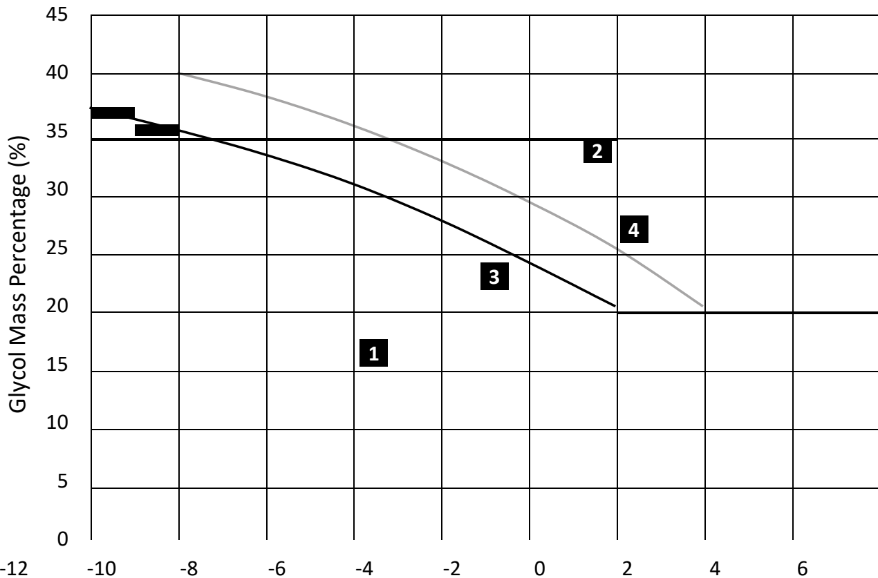
Figure 16 - Glycol percentage recommendation curve
