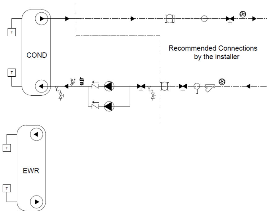
Figure 12b - Example of Hydronic Group Schematic Double Pump Package for Hot Water Exchanger
