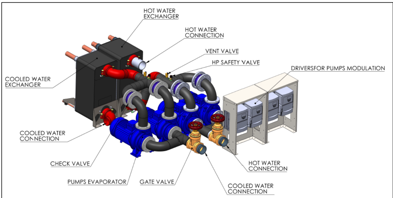
Figure 21 - Typical integrated chilled water pump
