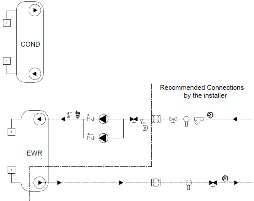
Figure 11b - Example of Hydronic Group Schematic Double Pump Package for chilled water exchanger
