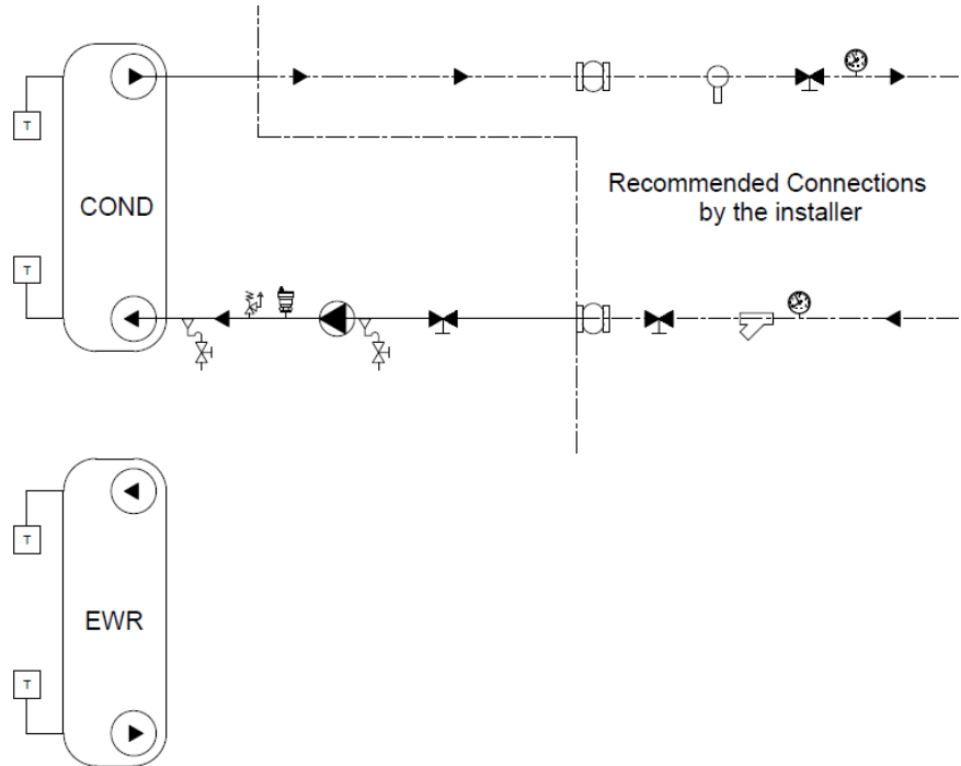
Figure 12 - Example of Hydronic Group Schematic Single Pump Package for Hot Water Exchanger
