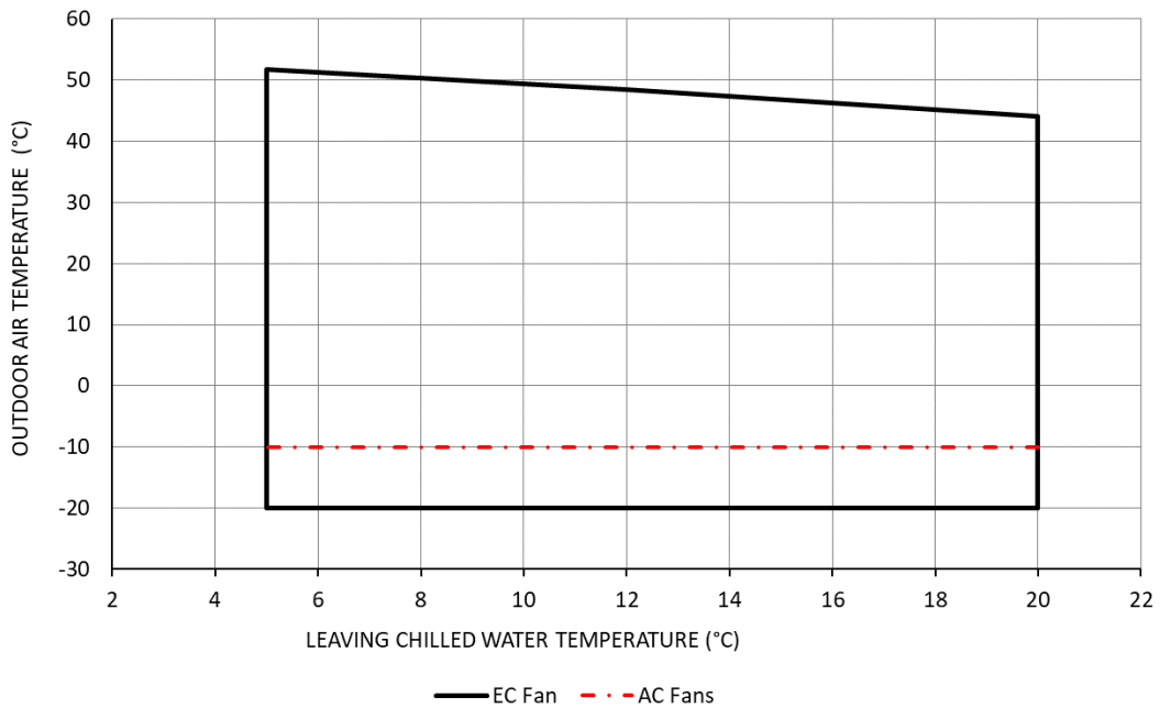
Figure 19 - Cooling operating map
