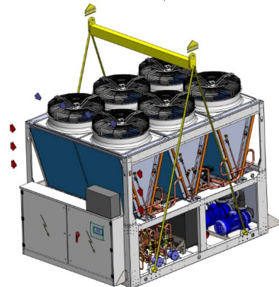
Figure 2 - Typical handling
